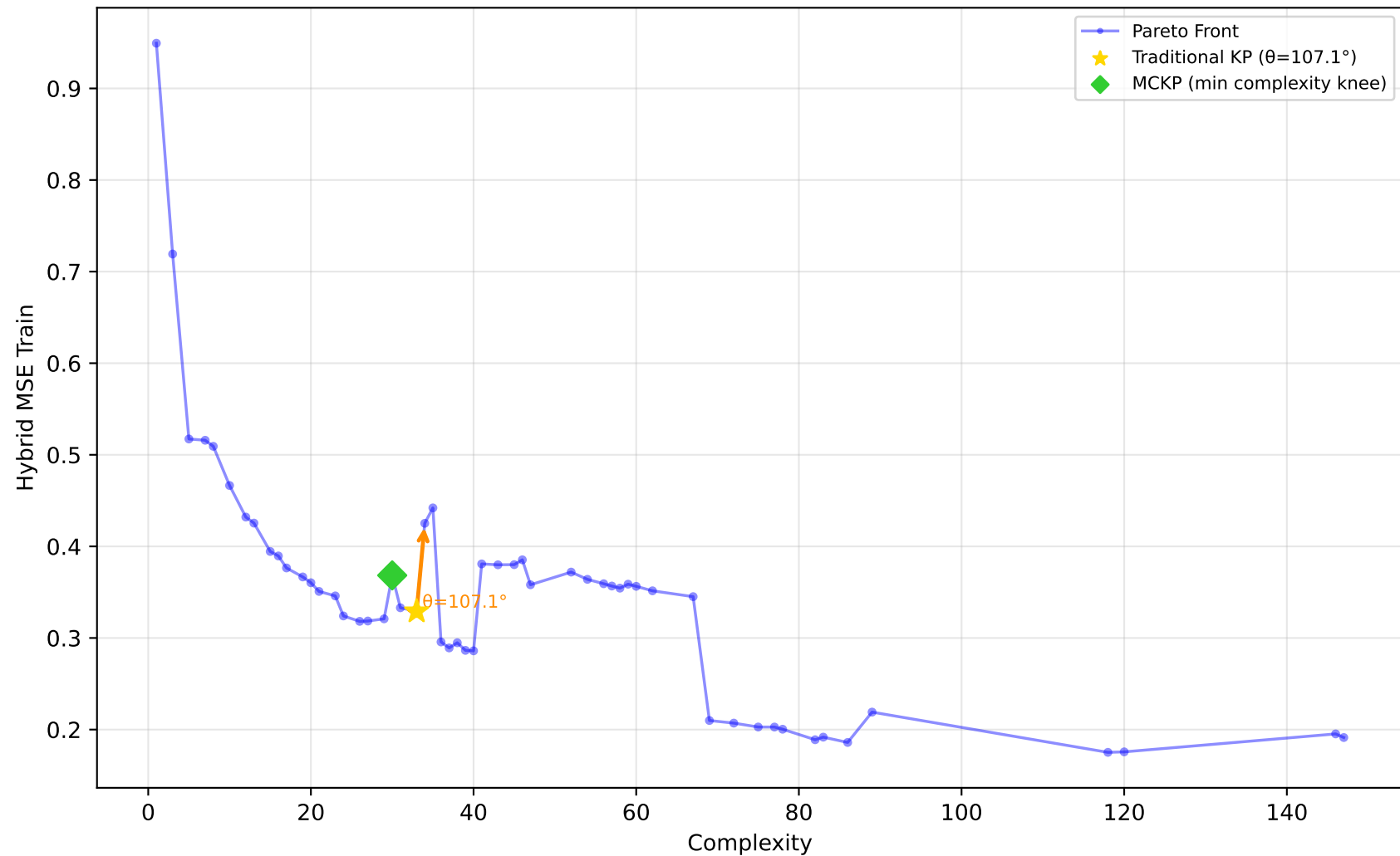
192_vineyard - Run 26 - MVP - Hybrid MSE Train \lambda_1=0.40, \lambda_2=0.00, \lambda_3=1.00 | Difficulty: 0.32 | Method: mckp
