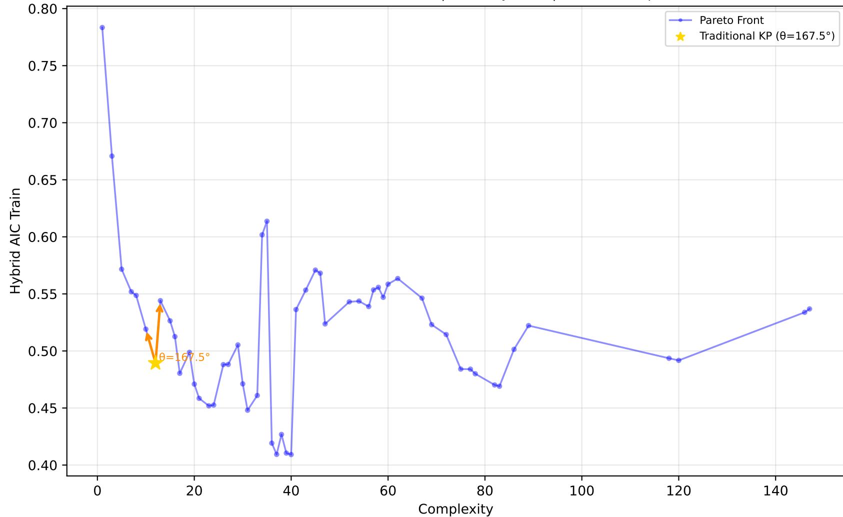
192_vineyard - Run 26 - SVP - Hybrid AIC Train \lambda_1=0.00, \lambda_2=1.00, \lambda_3=1.00 | Difficulty: 0.32 | Method: mckp
