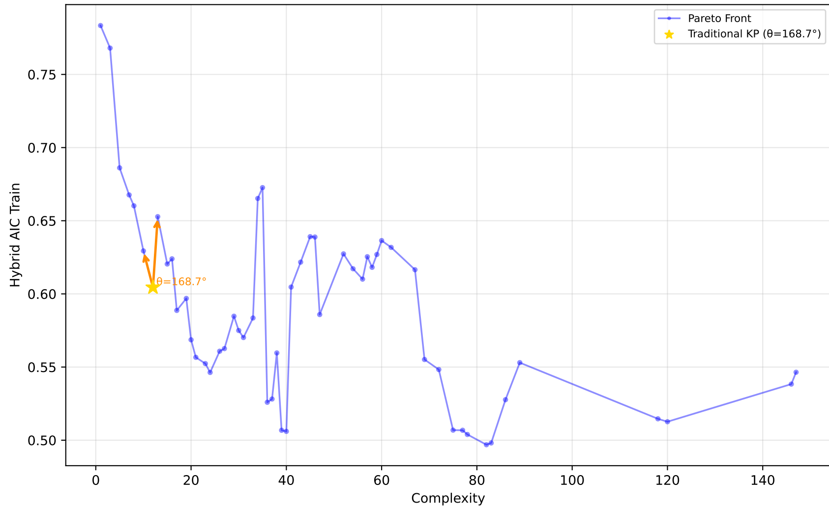
192_vineyard - Run 26 - SVP - Hybrid AIC Train \lambda_1=0.70, \lambda_2=0.70, \lambda_3=0.90 | Difficulty: 0.32 | Method: mckp
