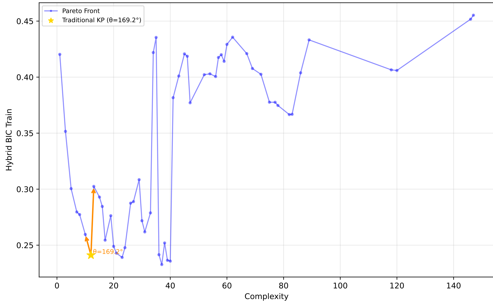
192_vineyard - Run 26 - SVP - Hybrid BIC Train \lambda_1=0.00, \lambda_2=1.00, \lambda_3=1.00 | Difficulty: 0.32 | Method: mckp
