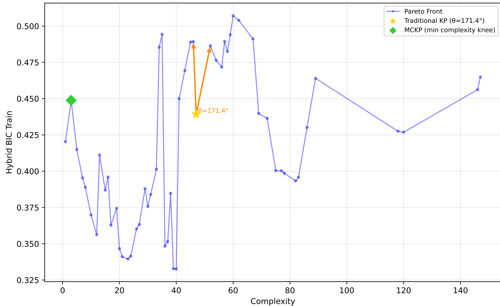
192_vineyard - Run 26 - SVP - Hybrid BIC Train \lambda_1=0.70, \lambda_2=0.70, \lambda_3=0.90 | Difficulty: 0.32 | Method: mckp
