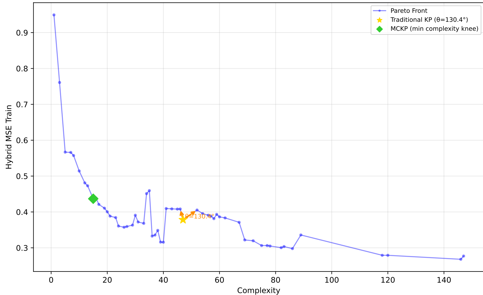
192_vineyard - Run 26 - SVP - Hybrid MSE Train \lambda_1=0.70, \lambda_2=0.70, \lambda_3=0.90 | Difficulty: 0.32 | Method: mckp
