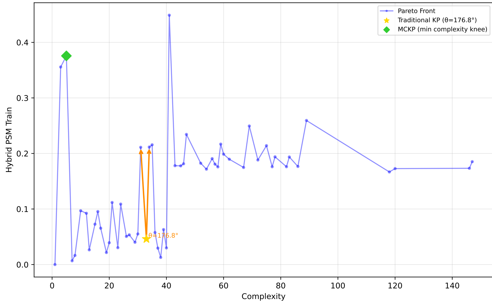
192_vineyard - Run 26 - SVP - Hybrid PSM Train \lambda_1=0.00, \lambda_2=1.00, \lambda_3=1.00 | Difficulty: 0.32 | Method: mckp
