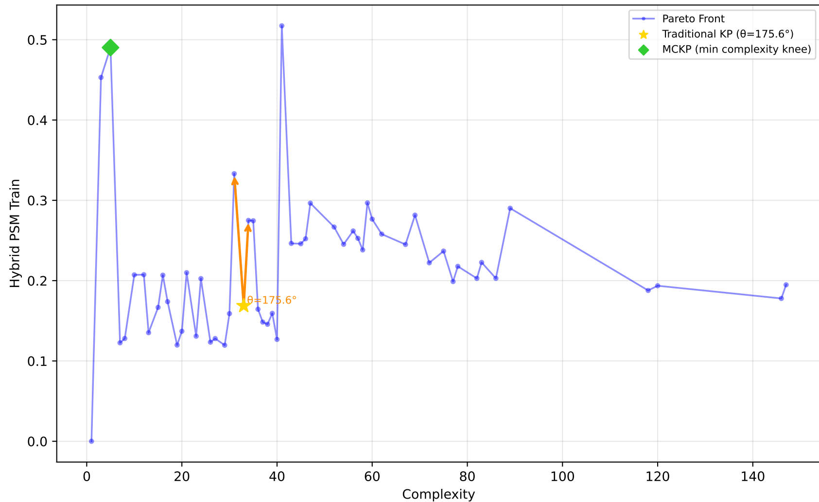
192_vineyard - Run 26 - SVP - Hybrid PSM Train \lambda_1=0.70, \lambda_2=0.70, \lambda_3=0.90 | Difficulty: 0.32 | Method: mckp
