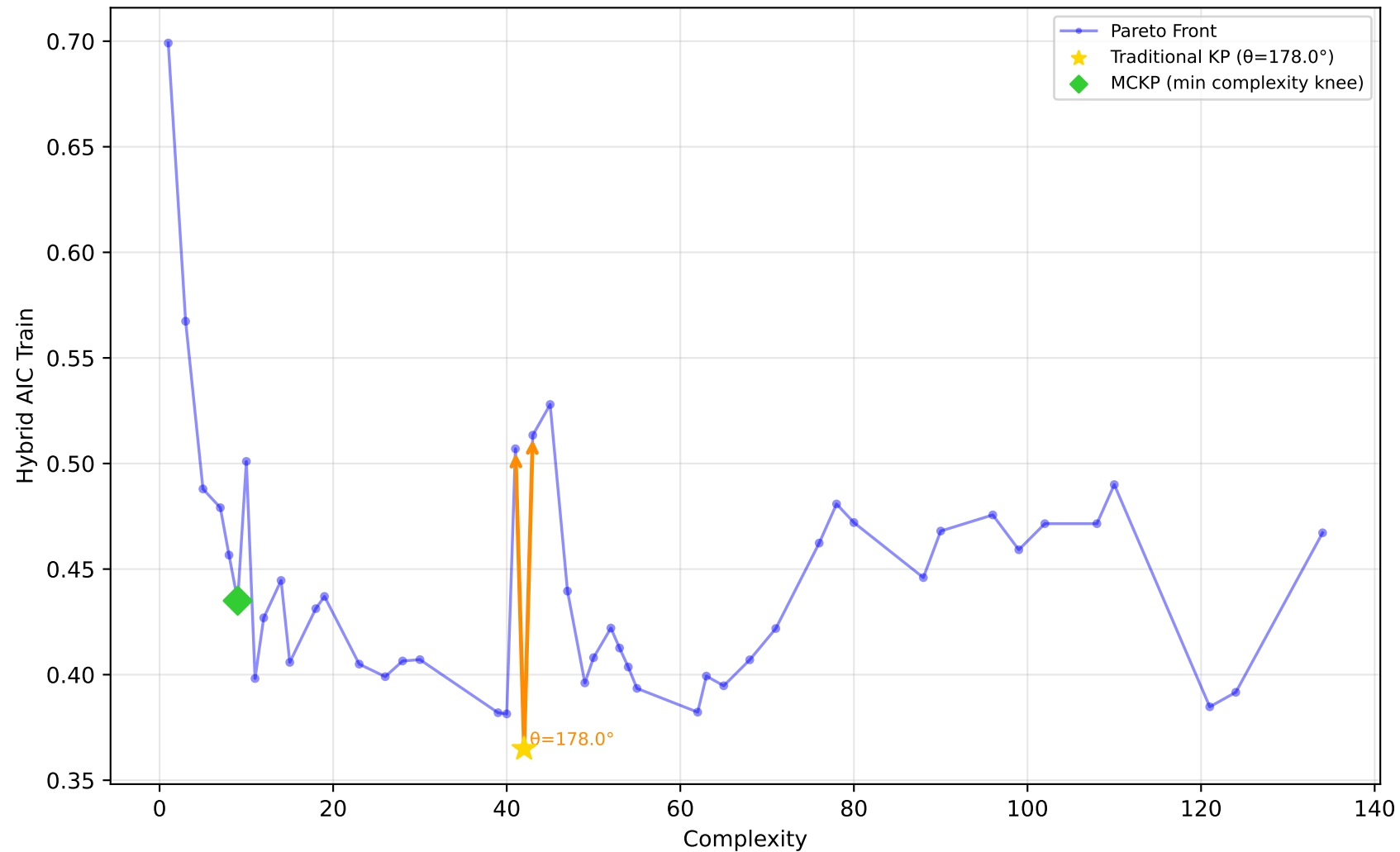
192_vineyard - Run 27 - MVP - Hybrid AIC Train \lambda_1=0.00, \bar{\lambda}_2=0.30, \lambda_3=1.00 | Difficulty: 0.73 | Method: hmr
