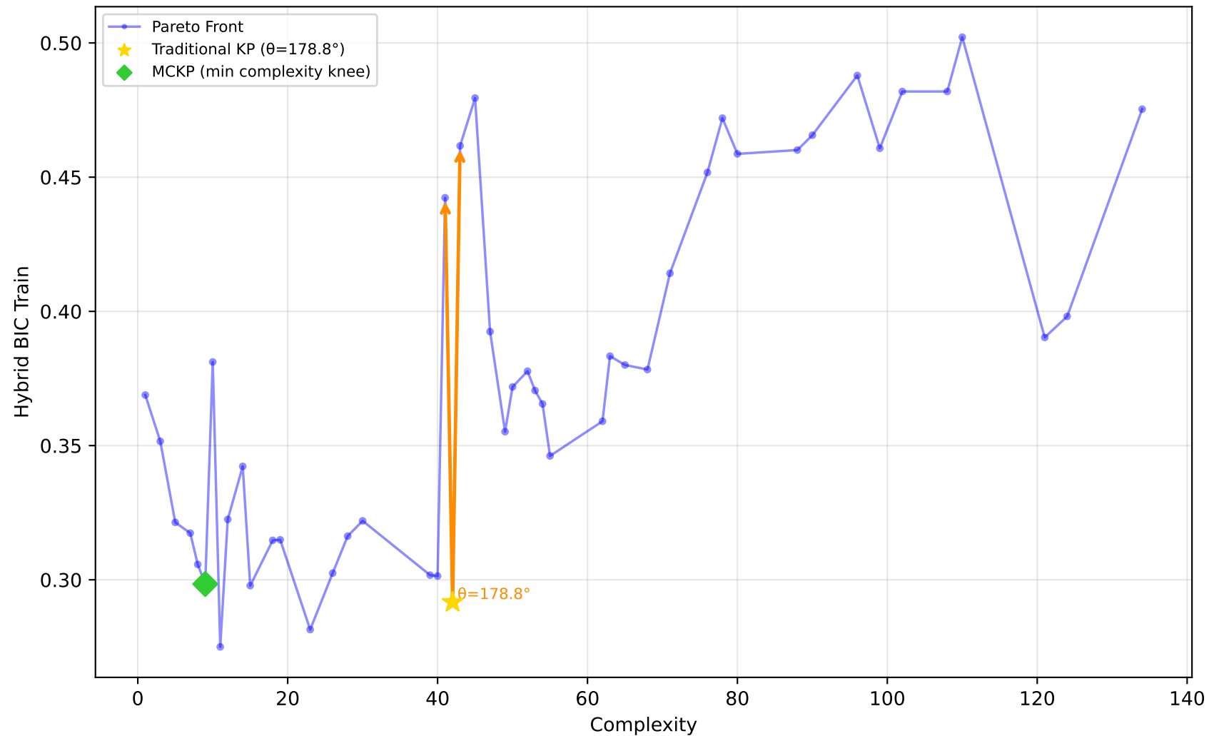
192_vineyard - Run 27 - MVP - Hybrid BIC Train \lambda_1=0.40, \bar{\lambda}_2=0.00, \lambda_3=1.00 | Difficulty: 0.73 | Method: hmr
