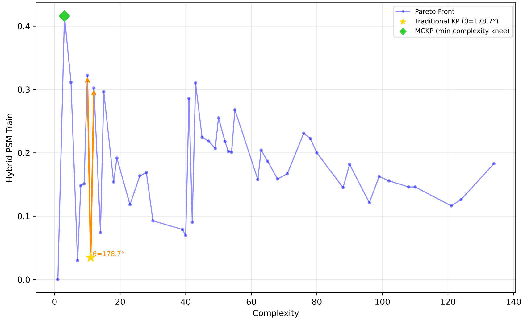
192_vineyard - Run 27 - MVP - Hybrid PSM Train \lambda_1=0.00, \bar{\lambda}_2=0.30, \lambda_3=1.00 | Difficulty: 0.73 | Method: hmr
