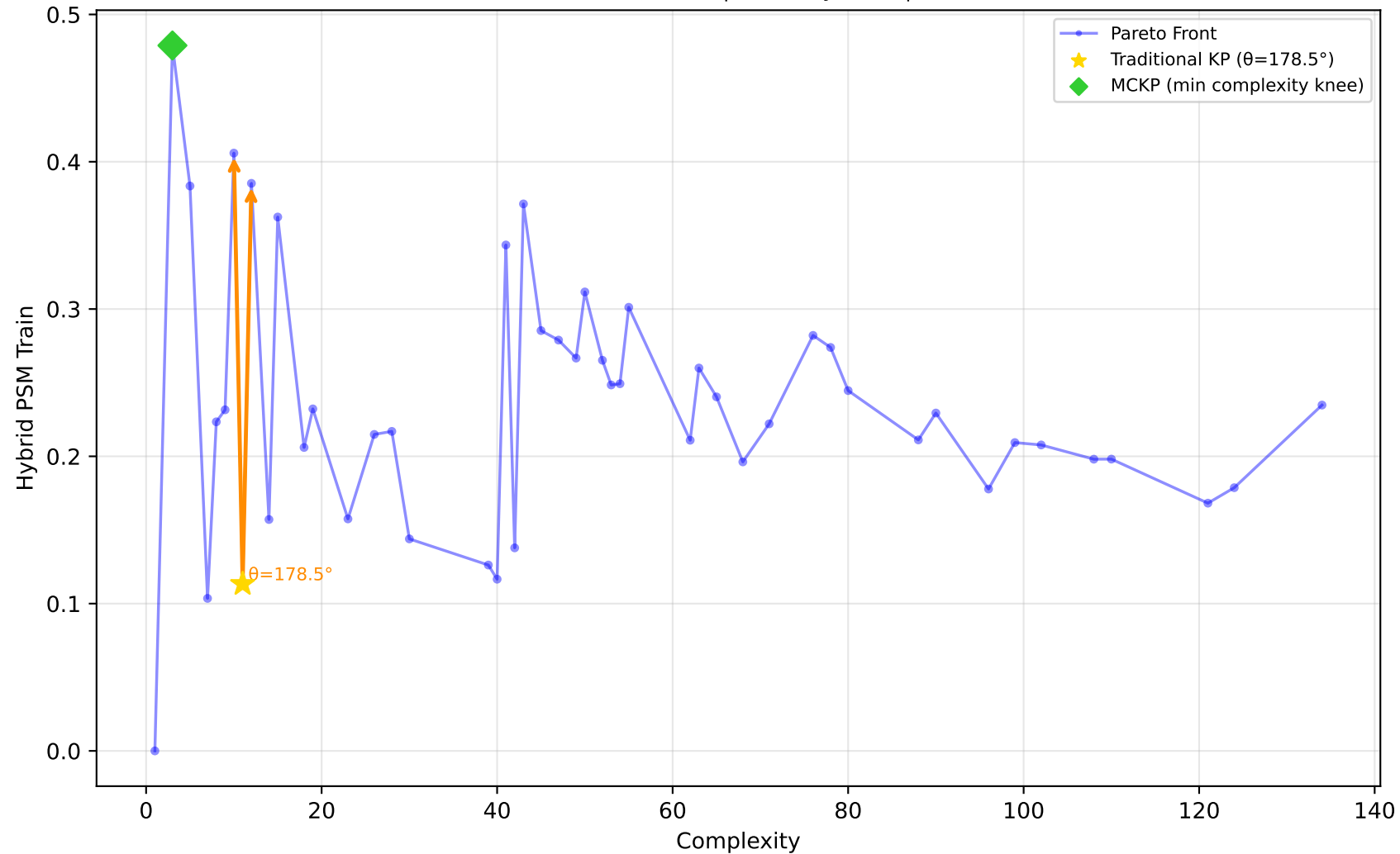
192_vineyard - Run 27 - MVP - Hybrid PSM Train \lambda_1=0.40, \bar{\lambda}_2=0.00, \lambda_3=1.00 | Difficulty: 0.73 | Method: hmr
