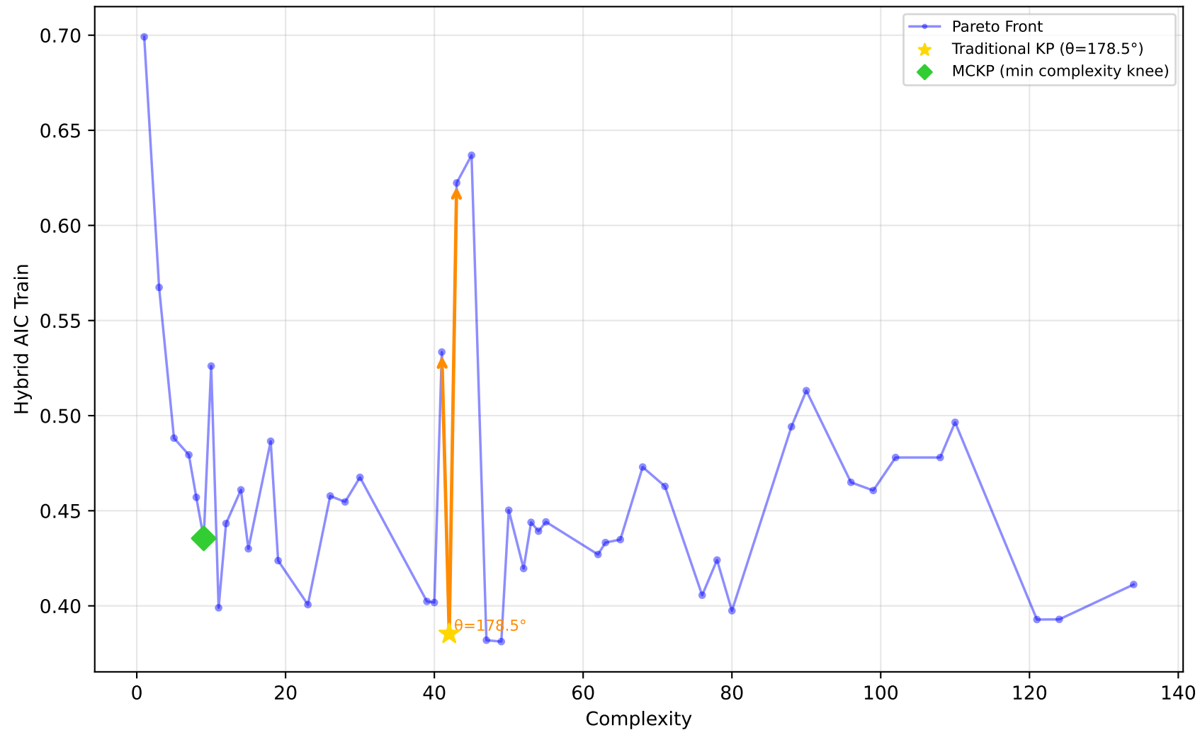
192_vineyard - Run 27 - SVP - Hybrid AIC Train \lambda_1=0.00, \bar{\lambda}_2=1.00, \lambda_3=1.00 | Difficulty: 0.73 | Method: hmr
