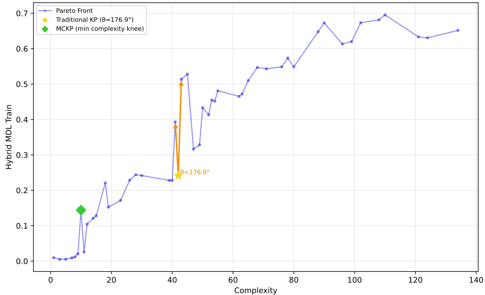
192_vineyard - Run 27 - SVP - Hybrid MDL Train \lambda_1=0.00, \bar{\lambda}_2=1.00, \lambda_3=1.00 | Difficulty: 0.73 | Method: hmr
