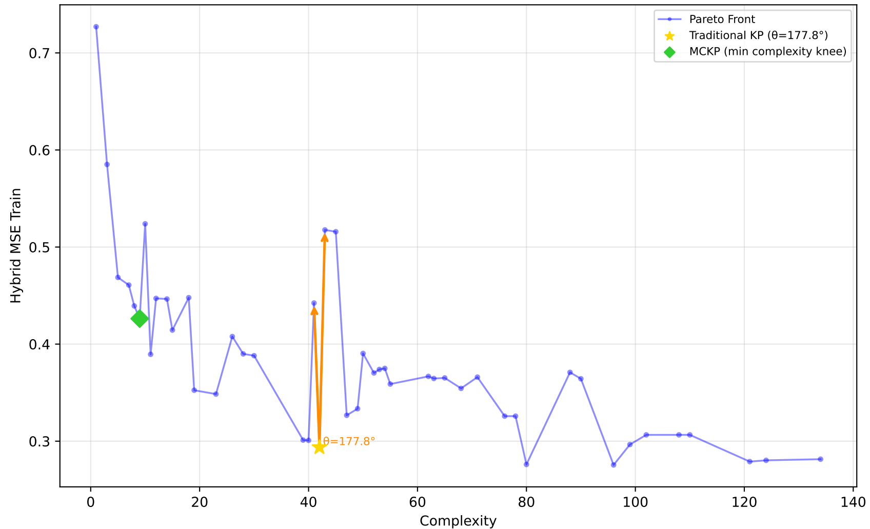
192_vineyard - Run 27 - SVP - Hybrid MSE Train \lambda_1=0.70, \bar{\lambda}_2=0.70, \lambda_3=0.90 | Difficulty: 0.73 | Method: hmr
