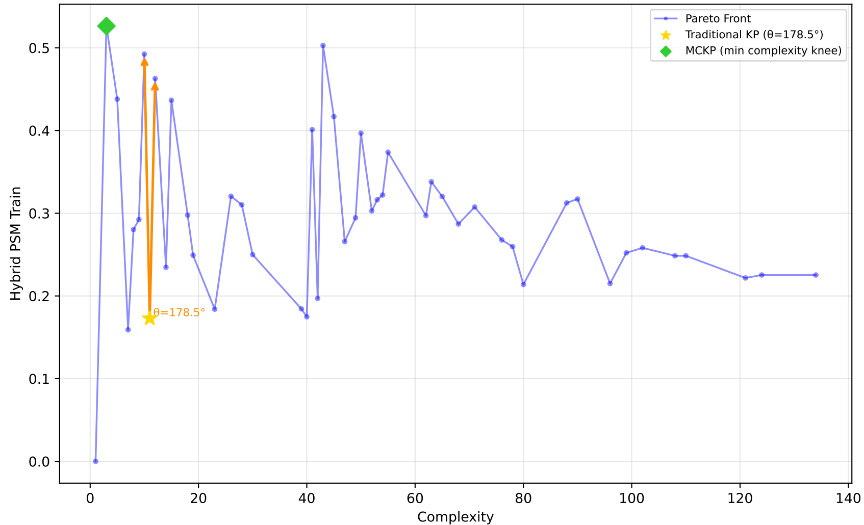
192_vineyard - Run 27 - SVP - Hybrid PSM Train \lambda_1=0.70, \bar{\lambda}_2=0.70, \lambda_3=0.90 | Difficulty: 0.73 | Method: hmr
