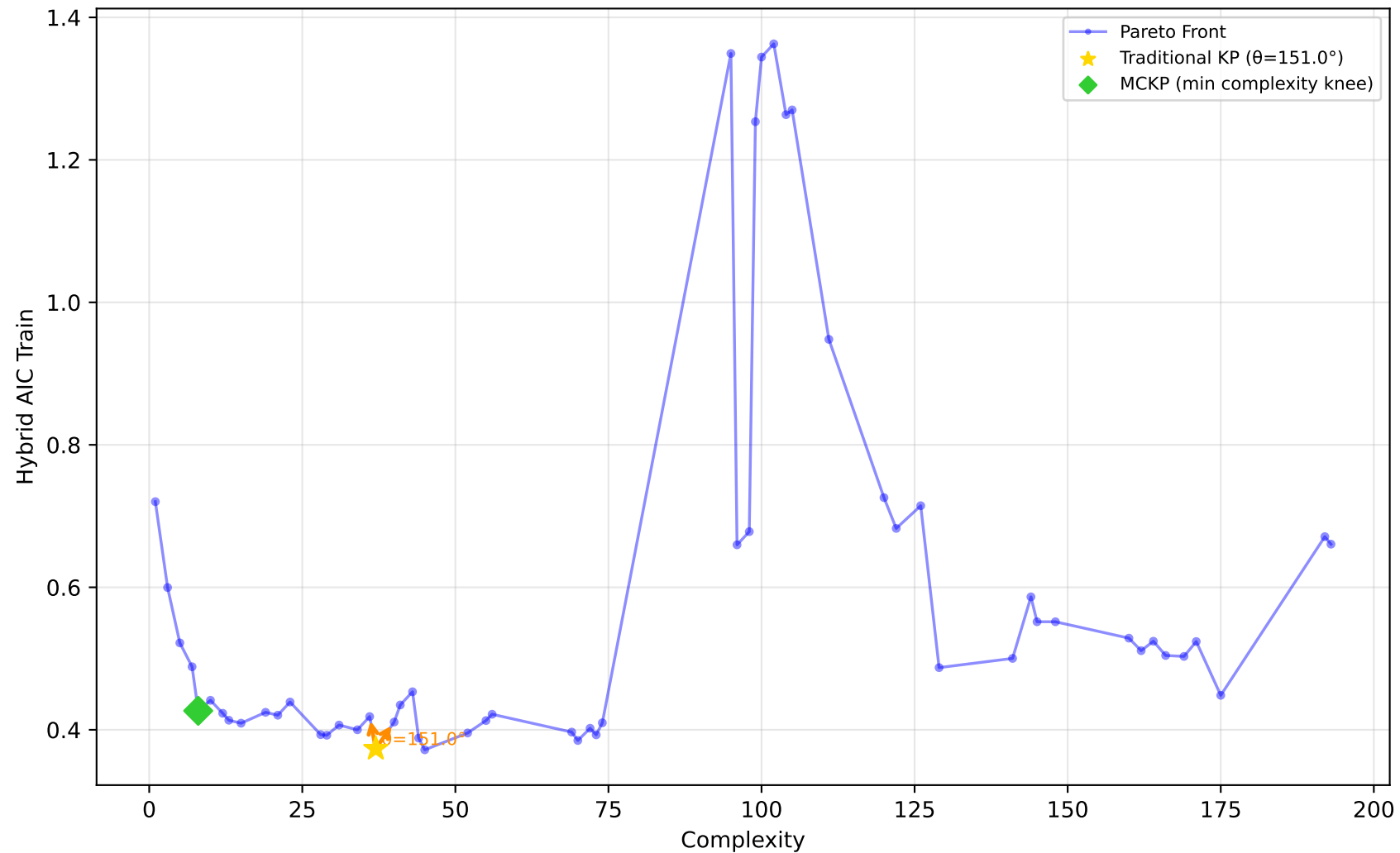
192_vineyard - Run 28 - MVP - Hybrid AIC Train \lambda_1=0.00, \lambda_2=0.30, \lambda_3=1.00 | Difficulty: 1.00 | Method: hmr
