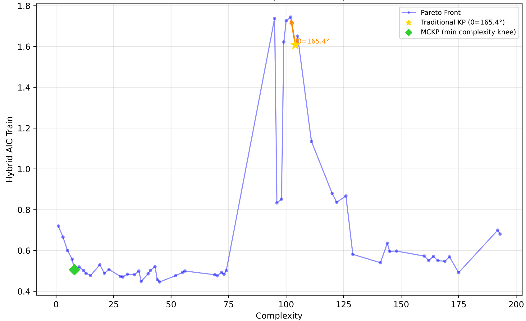
192_vineyard - Run 28 - MVP - Hybrid AIC Train \lambda_1=0.40, \bar{\lambda}_2=0.00, \lambda_3=1.00 | Difficulty: 1.00 | Method: hmr
