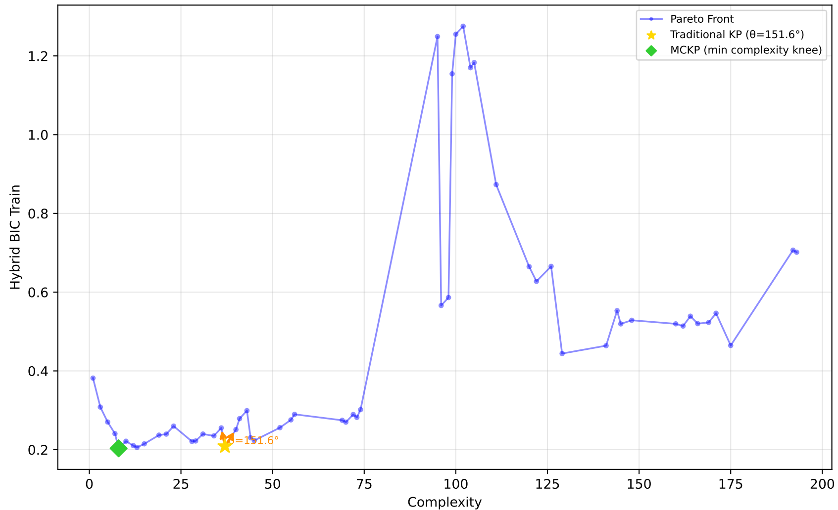
192_vineyard - Run 28 - MVP - Hybrid BIC Train \lambda_1=0.00, \lambda_2=0.30, \lambda_3=1.00 | Difficulty: 1.00 | Method: hmr
