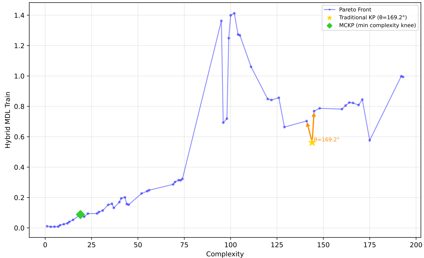
192_vineyard - Run 28 - MVP - Hybrid MDL Train \lambda_1=0.00, \bar{\lambda}_2=0.30, \lambda_3=1.00 | Difficulty: 1.00 | Method: hmr
