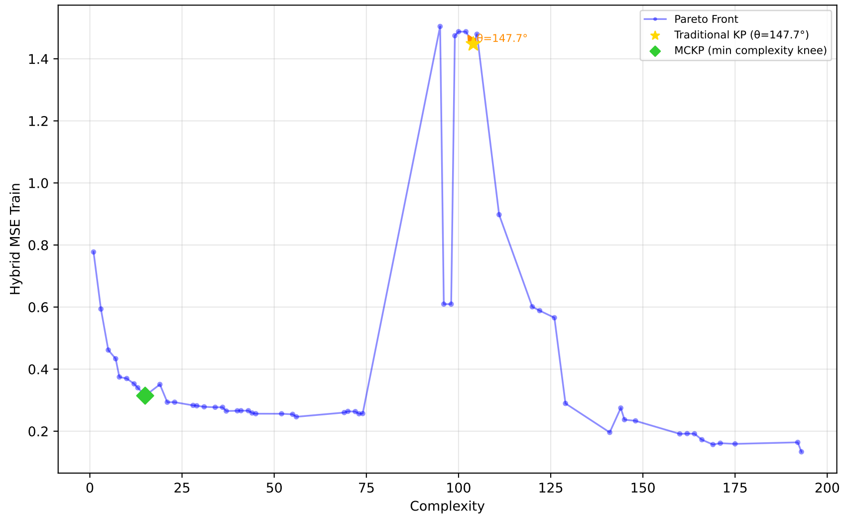
192_vineyard - Run 28 - MVP - Hybrid MSE Train \lambda_1=0.40, \bar{\lambda}_2=0.00, \lambda_3=1.00 | Difficulty: 1.00 | Method: hmr
