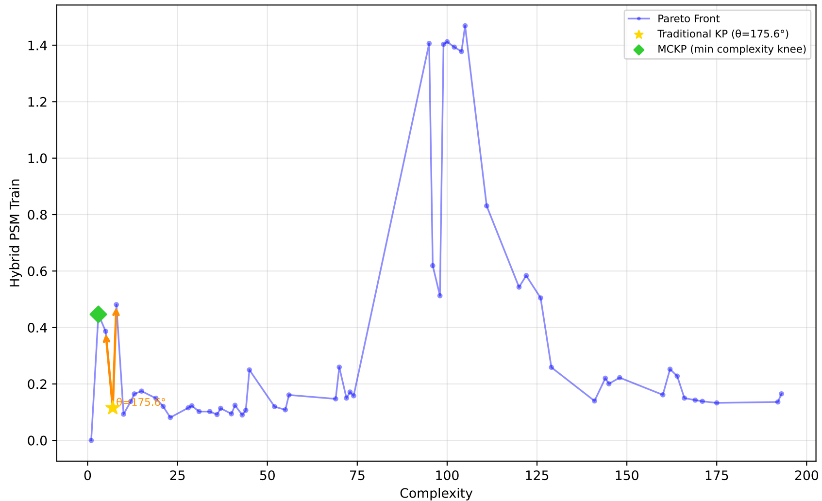
192_vineyard - Run 28 - MVP - Hybrid PSM Train \lambda_1=0.40, \bar{\lambda}_2=0.00, \lambda_3=1.00 | Difficulty: 1.00 | Method: hmr
