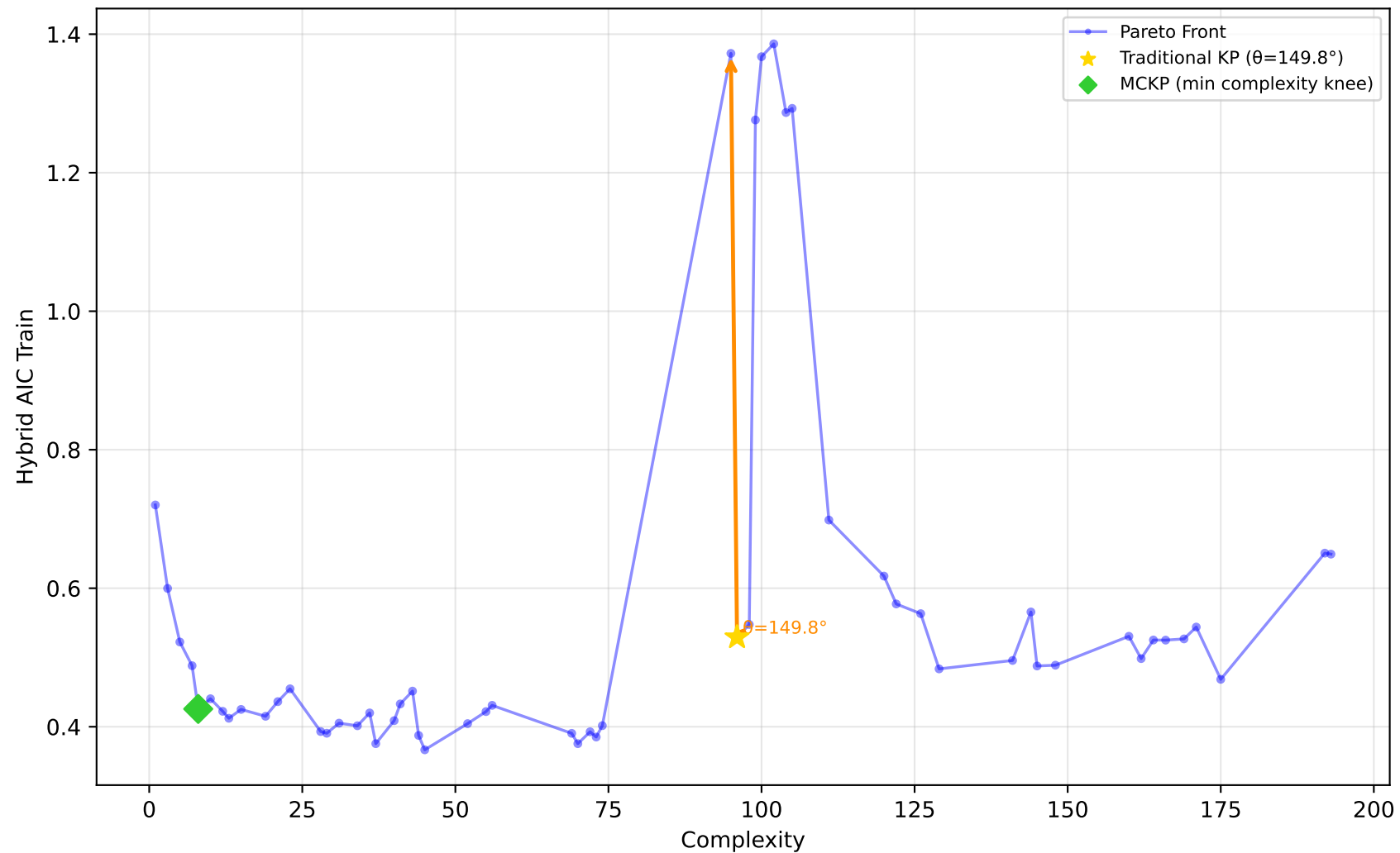
192_vineyard - Run 28 - SVP - Hybrid AIC Train \lambda_1=0.00, \bar{\lambda}_2=1.00, \lambda_3=1.00 | Difficulty: 1.00 | Method: hmr
