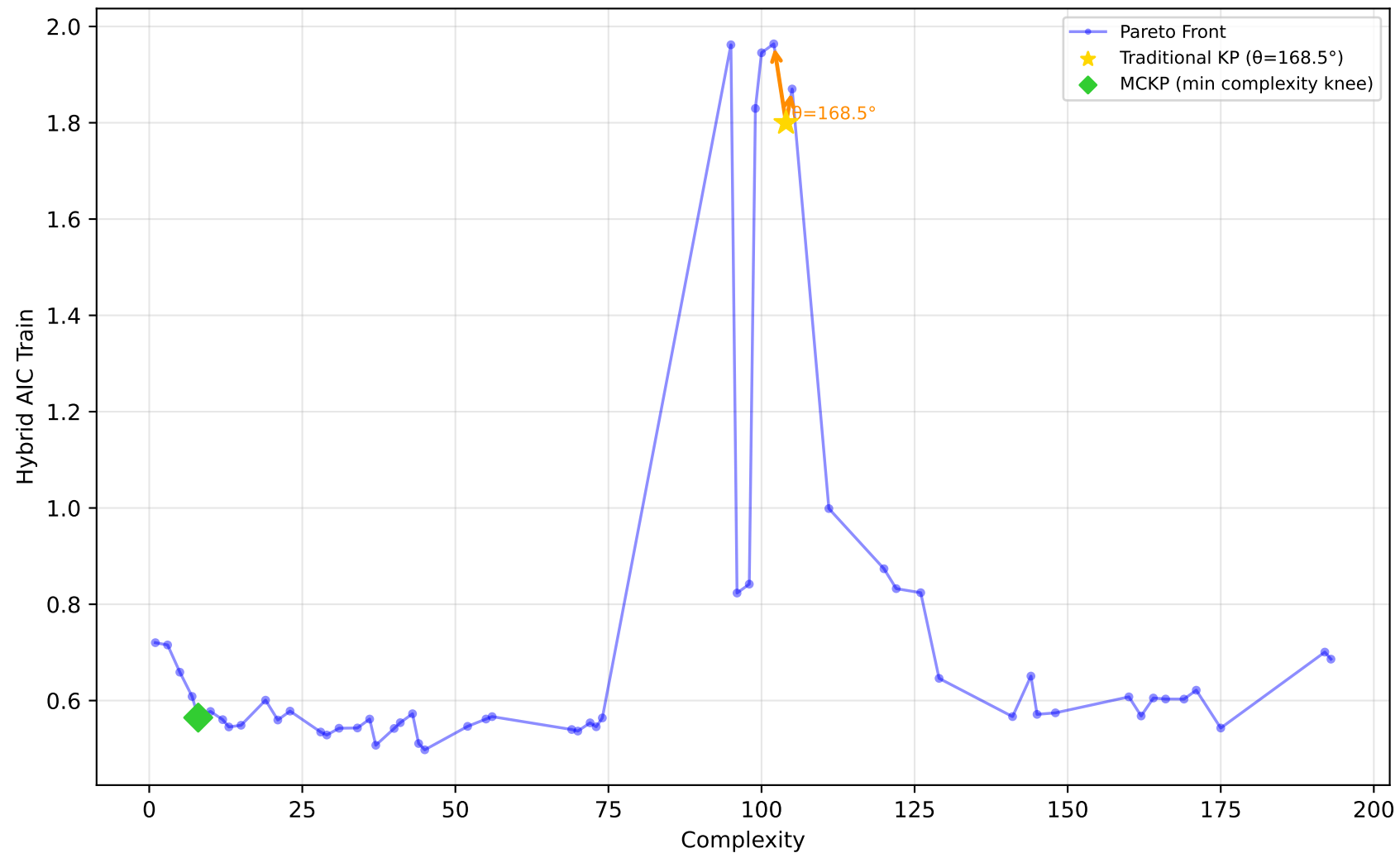
192_vineyard - Run 28 - SVP - Hybrid AIC Train \lambda_1=0.70, \bar{\lambda}_2=0.70, \lambda_3=0.90 | Difficulty: 1.00 | Method: hmr
