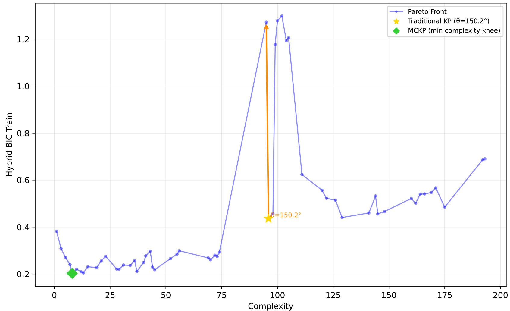
192_vineyard - Run 28 - SVP - Hybrid BIC Train \lambda_1=0.00, \bar{\lambda}_2=1.00, \lambda_3=1.00 | Difficulty: 1.00 | Method: hmr
