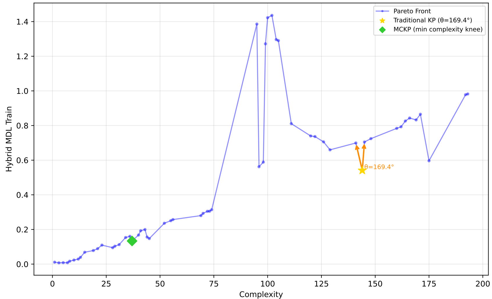
192_vineyard - Run 28 - SVP - Hybrid MDL Train \lambda_1=0.00, \bar{\lambda}_2=1.00, \lambda_3=1.00 | Difficulty: 1.00 | Method: hmr
