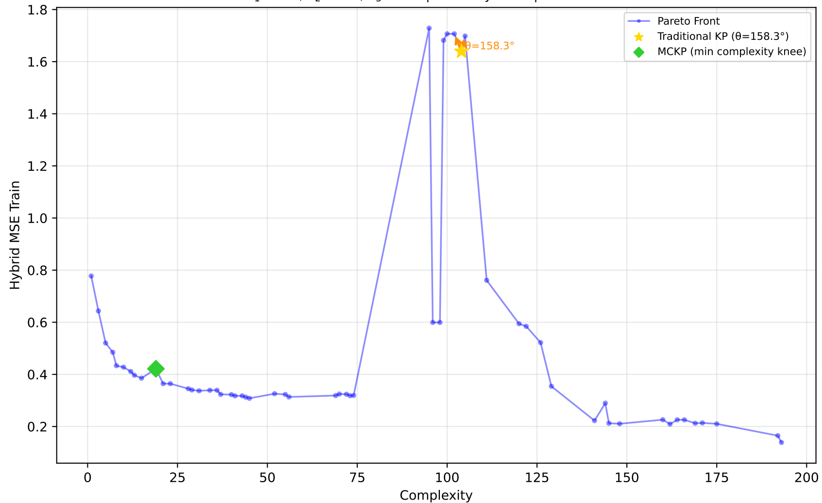
192_vineyard - Run 28 - SVP - Hybrid MSE Train \lambda_1=0.70, \lambda_2=0.70, \lambda_3=0.90 | Difficulty: 1.00 | Method: hmr
