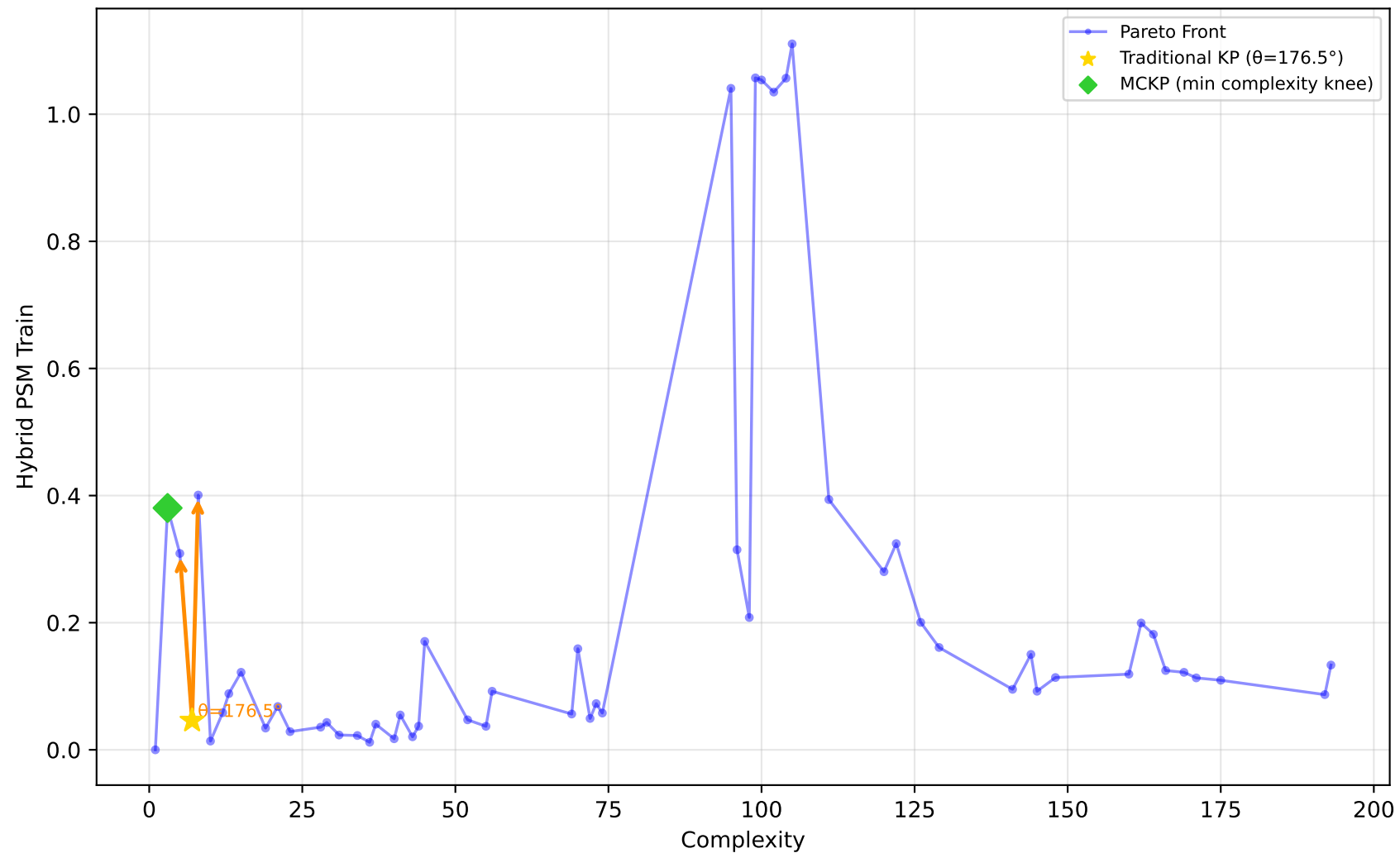
192_vineyard - Run 28 - SVP - Hybrid PSM Train \lambda_1=0.00, \lambda_2=1.00, \lambda_3=1.00 | Difficulty: 1.00 | Method: hmr
