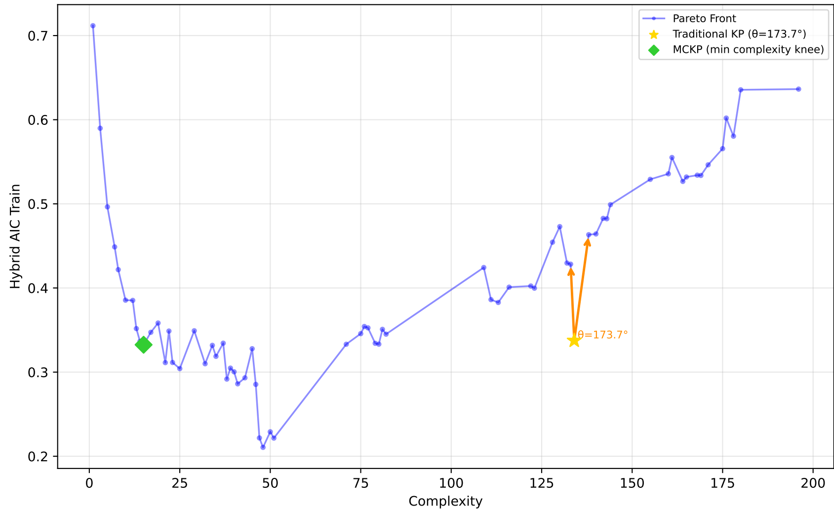
192_vineyard - Run 29 - MVP - Hybrid AIC Train \lambda_1=0.00, \bar{\lambda}_2=0.30, \lambda_3=1.00 | Difficulty: 0.88 | Method: hmr
