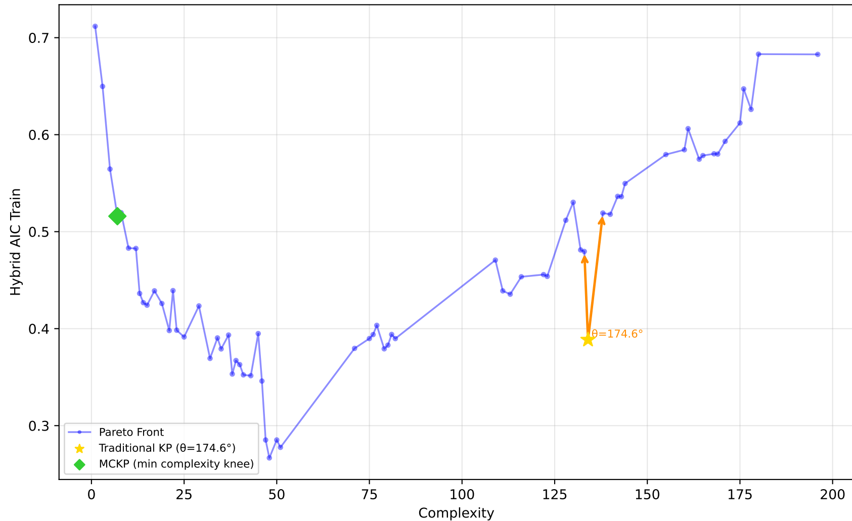
192_vineyard - Run 29 - MVP - Hybrid AIC Train \lambda_1=0.40, \bar{\lambda}_2=0.00, \lambda_3=1.00 | Difficulty: 0.88 | Method: hmr
