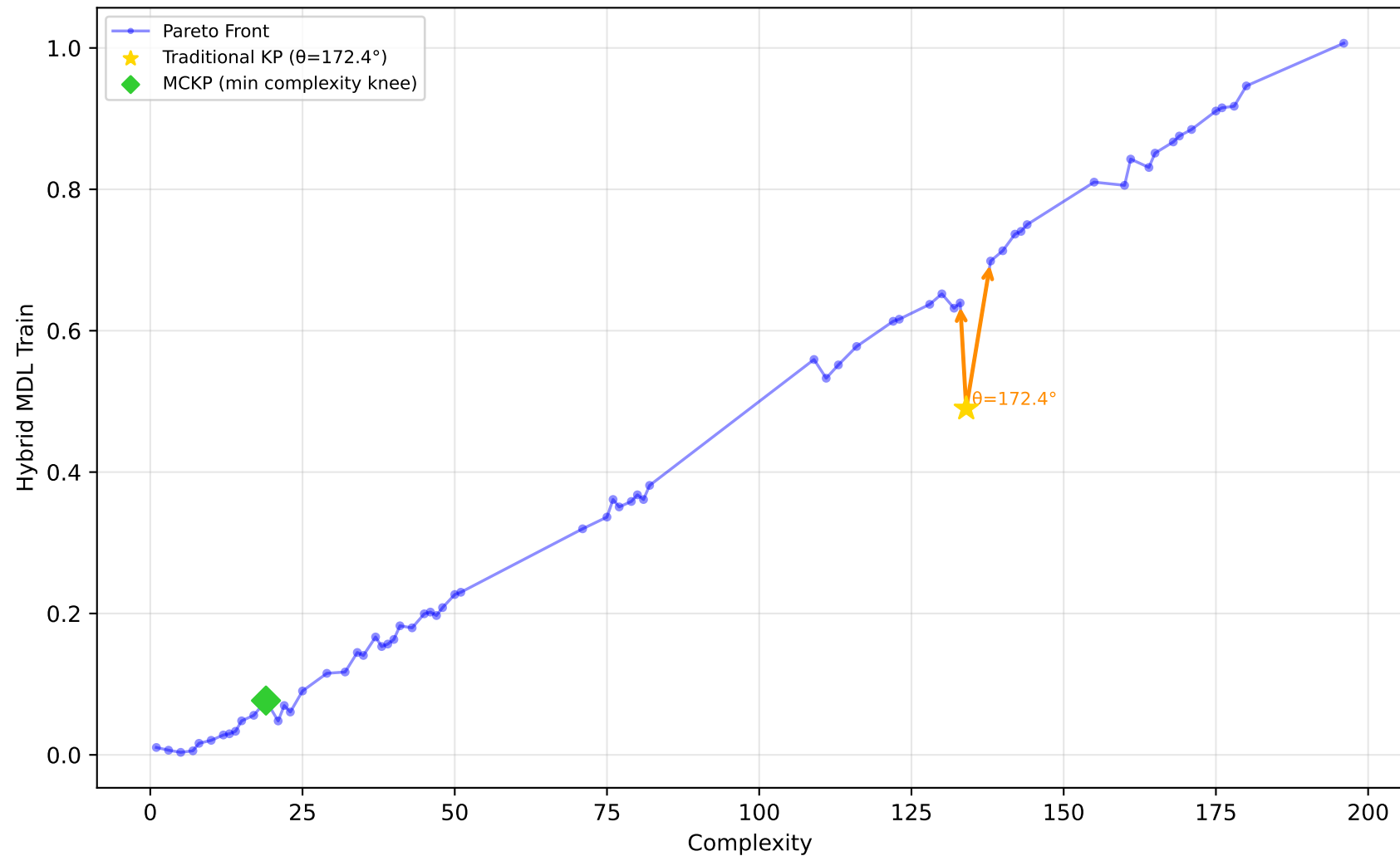
192_vineyard - Run 29 - MVP - Hybrid MDL Train \lambda_1=0.00, \lambda_2=0.30, \lambda_3=1.00 | Difficulty: 0.88 | Method: hmr
