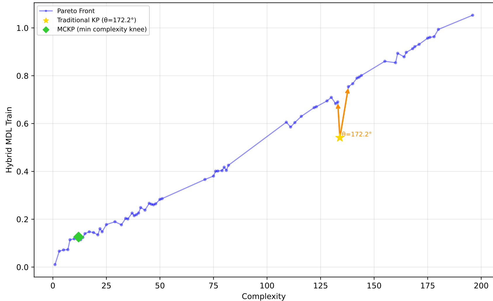
192_vineyard - Run 29 - MVP - Hybrid MDL Train \lambda_1=0.40, \lambda_2=0.00, \lambda_3=1.00 | Difficulty: 0.88 | Method: hmr
