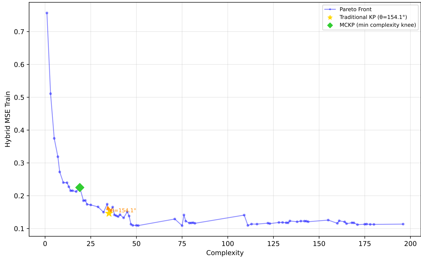
192_vineyard - Run 29 - MVP - Hybrid MSE Train \lambda_1=0.00, \lambda_2=0.30, \lambda_3=1.00 | Difficulty: 0.88 | Method: hmr
