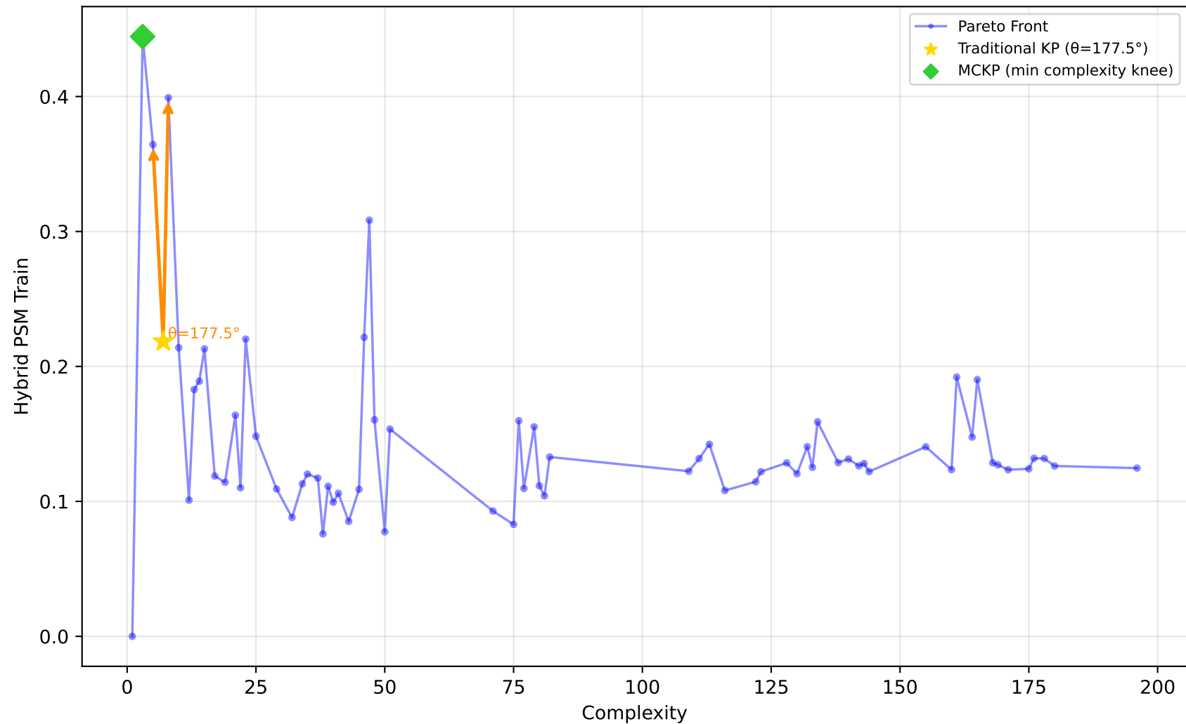
192_vineyard - Run 29 - MVP - Hybrid PSM Train \lambda_1=0.40, \lambda_2=0.00, \lambda_3=1.00 | Difficulty: 0.88 | Method: hmr
