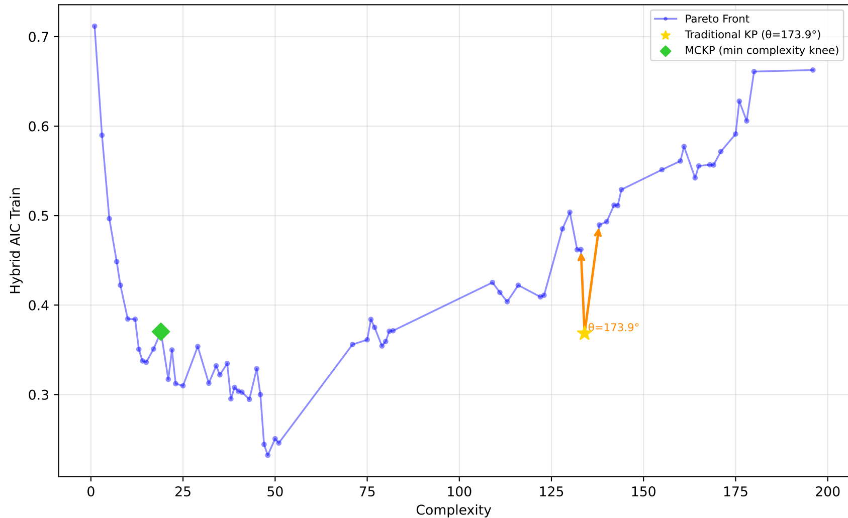
192_vineyard - Run 29 - SVP - Hybrid AIC Train \lambda_1=0.00, \bar{\lambda}_2=1.00, \lambda_3=1.00 | Difficulty: 0.88 | Method: hmr
