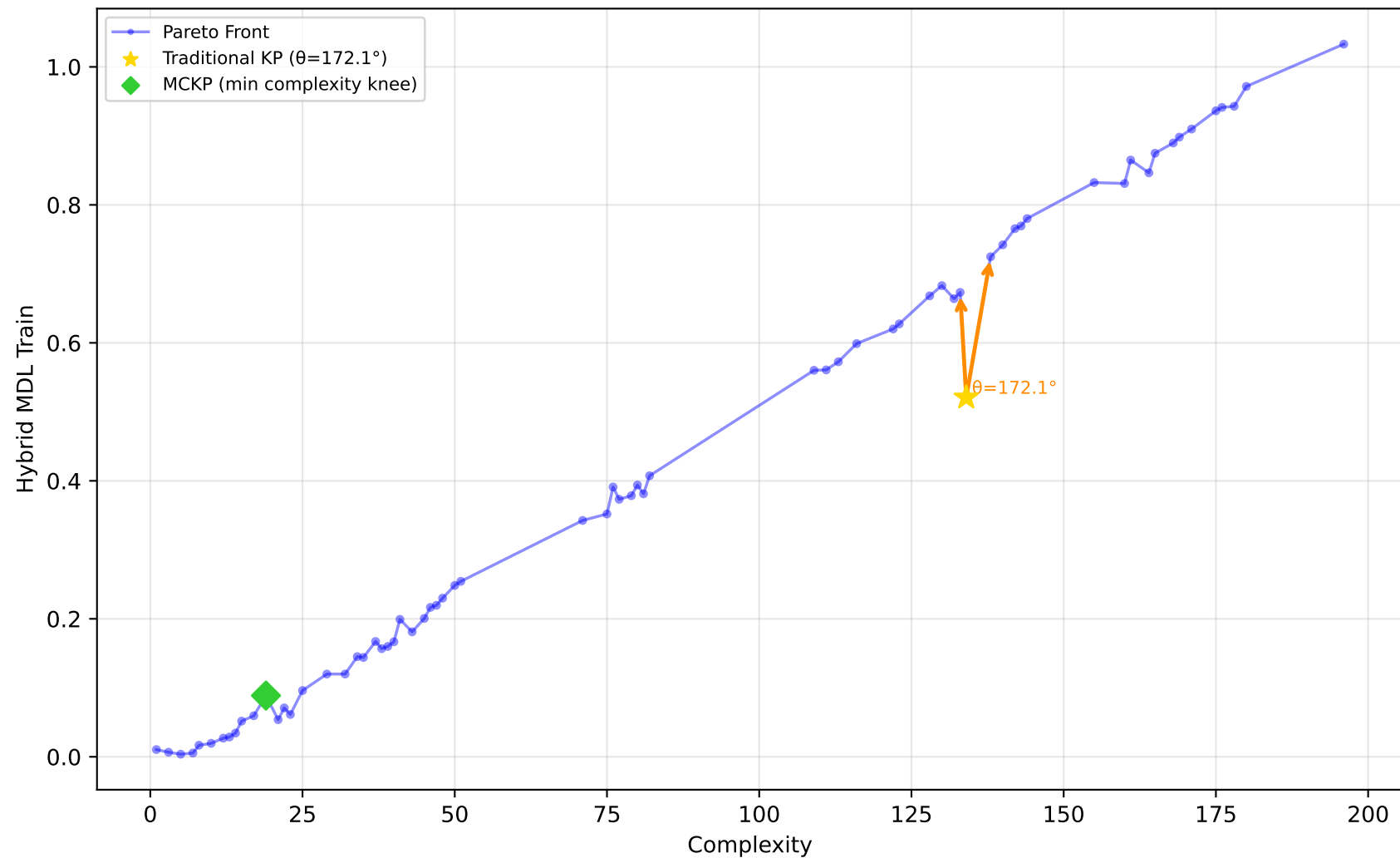
192_vineyard - Run 29 - SVP - Hybrid MDL Train \lambda_1=0.00, \lambda_2=1.00, \lambda_3=1.00 | Difficulty: 0.88 | Method: hmr
