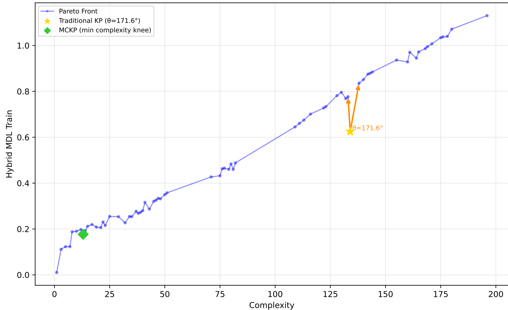
192_vineyard - Run 29 - SVP - Hybrid MDL Train \lambda_1=0.70, \bar{\lambda}_2=0.70, \lambda_3=0.90 | Difficulty: 0.88 | Method: hmr
