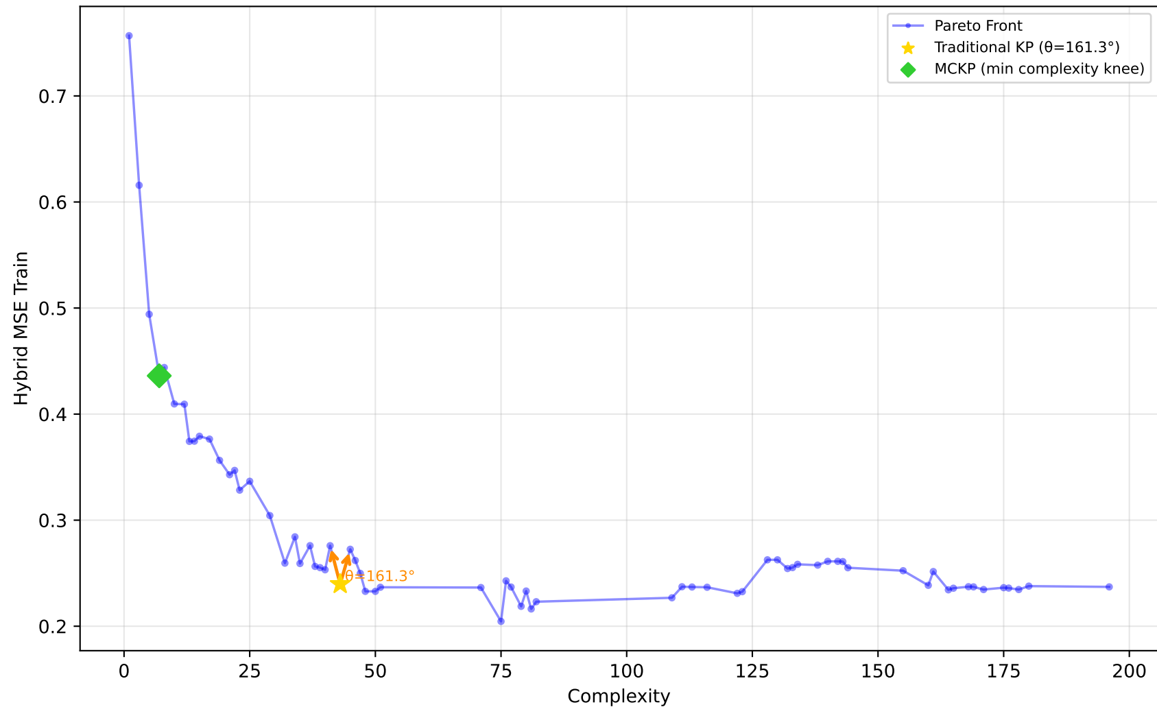
192_vineyard - Run 29 - SVP - Hybrid MSE Train \lambda_1=0.70, \bar{\lambda}_2=0.70, \lambda_3=0.90 | Difficulty: 0.88 | Method: hmr
