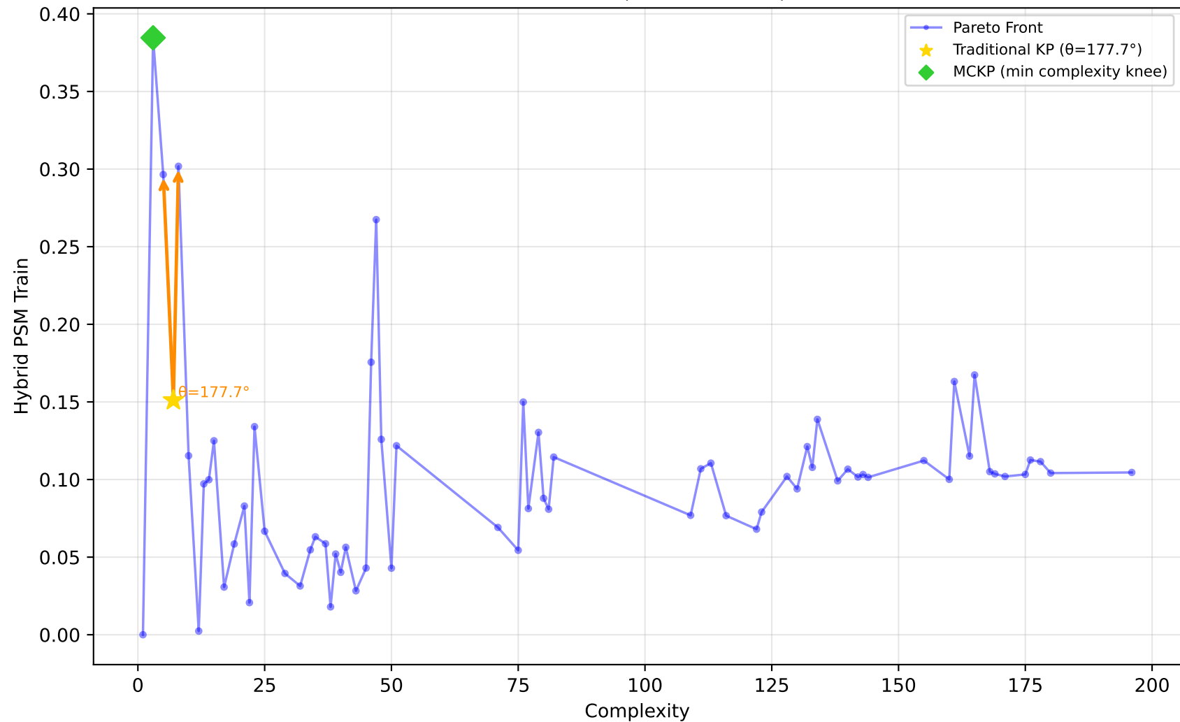
192_vineyard - Run 29 - SVP - Hybrid PSM Train \lambda_1=0.00, \bar{\lambda}_2=1.00, \lambda_3=1.00 | Difficulty: 0.88 | Method: hmr
