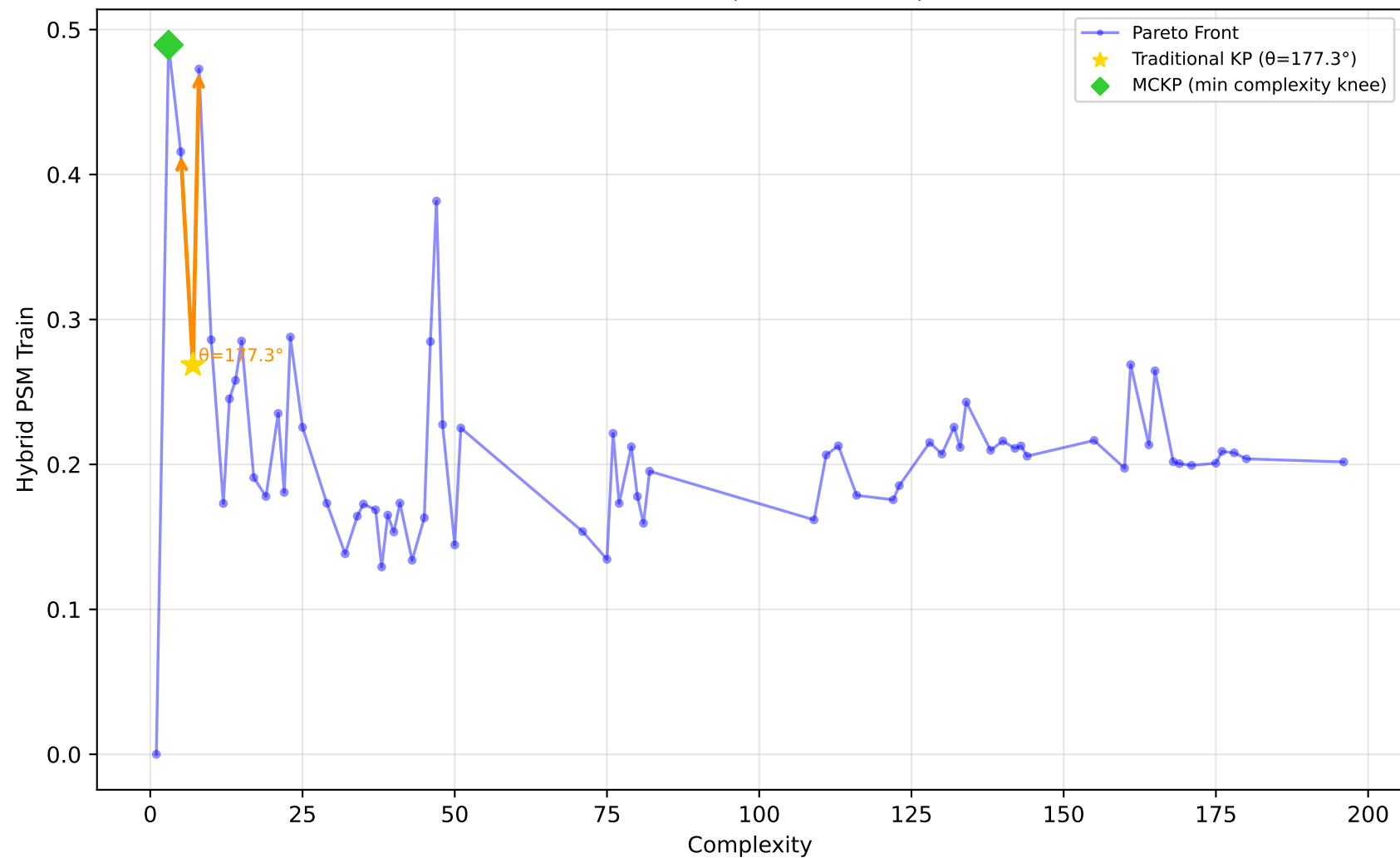
192_vineyard - Run 29 - SVP - Hybrid PSM Train \lambda_1=0.70, \bar{\lambda}_2=0.70, \lambda_3=0.90 | Difficulty: 0.88 | Method: hmr
