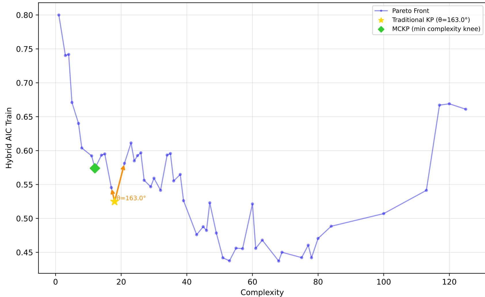
192_vineyard - Run 2 - MVP - Hybrid AIC Train \lambda_1=0.40, \lambda_2=0.00, \lambda_3=1.00 | Difficulty: 0.13 | Method: mckp
