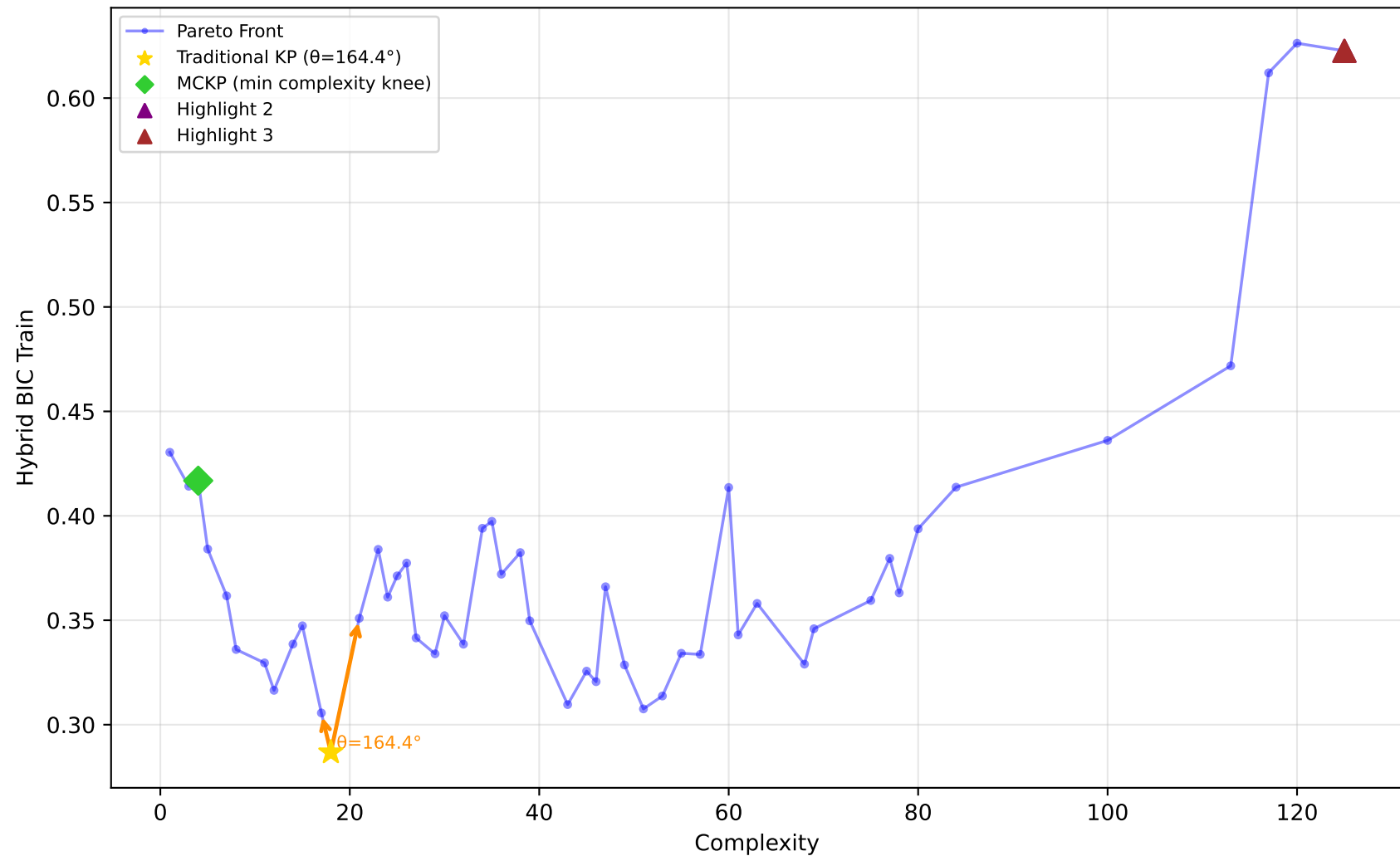
192_vineyard - Run 2 - MVP - Hybrid BIC Train \lambda_1=0.40, \lambda_2=0.00, \lambda_3=1.00 | Difficulty: 0.13 | Method: mckp
