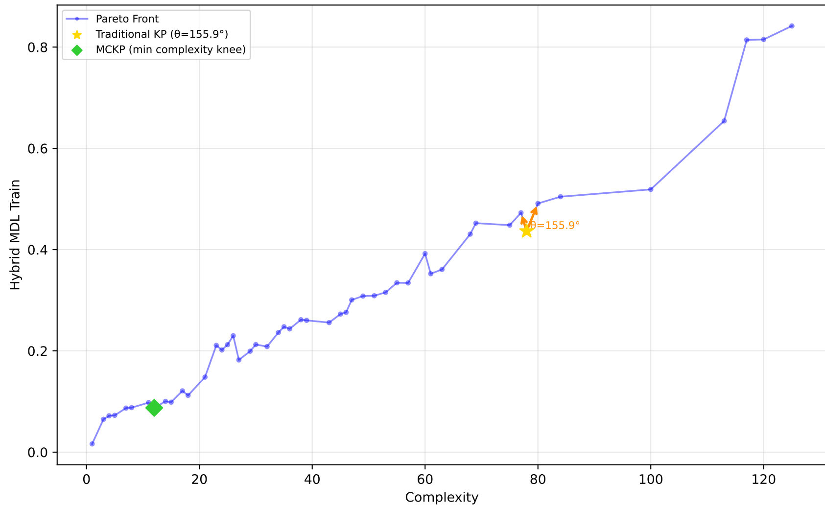
192_vineyard - Run 2 - MVP - Hybrid MDL Train \lambda_1=0.40, \lambda_2=0.00, \lambda_3=1.00 | Difficulty: 0.13 | Method: mckp
