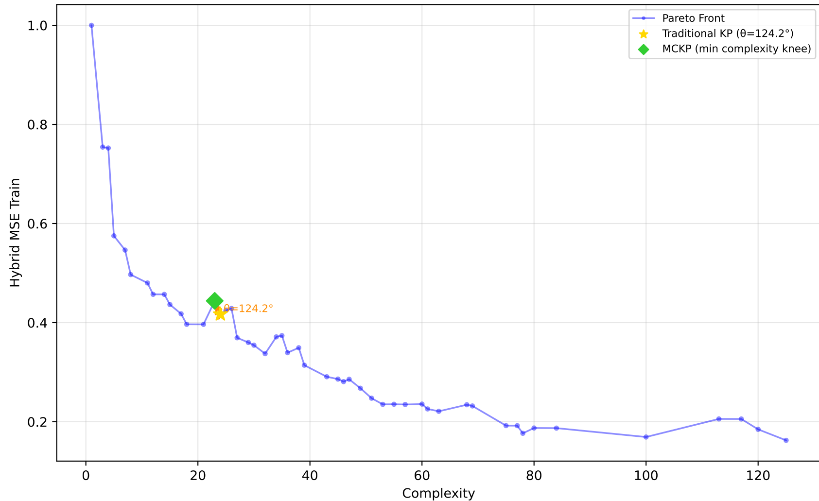
192_vineyard - Run 2 - MVP - Hybrid MSE Train \lambda_1=0.40, \lambda_2=0.00, \lambda_3=1.00 | Difficulty: 0.13 | Method: mckp
