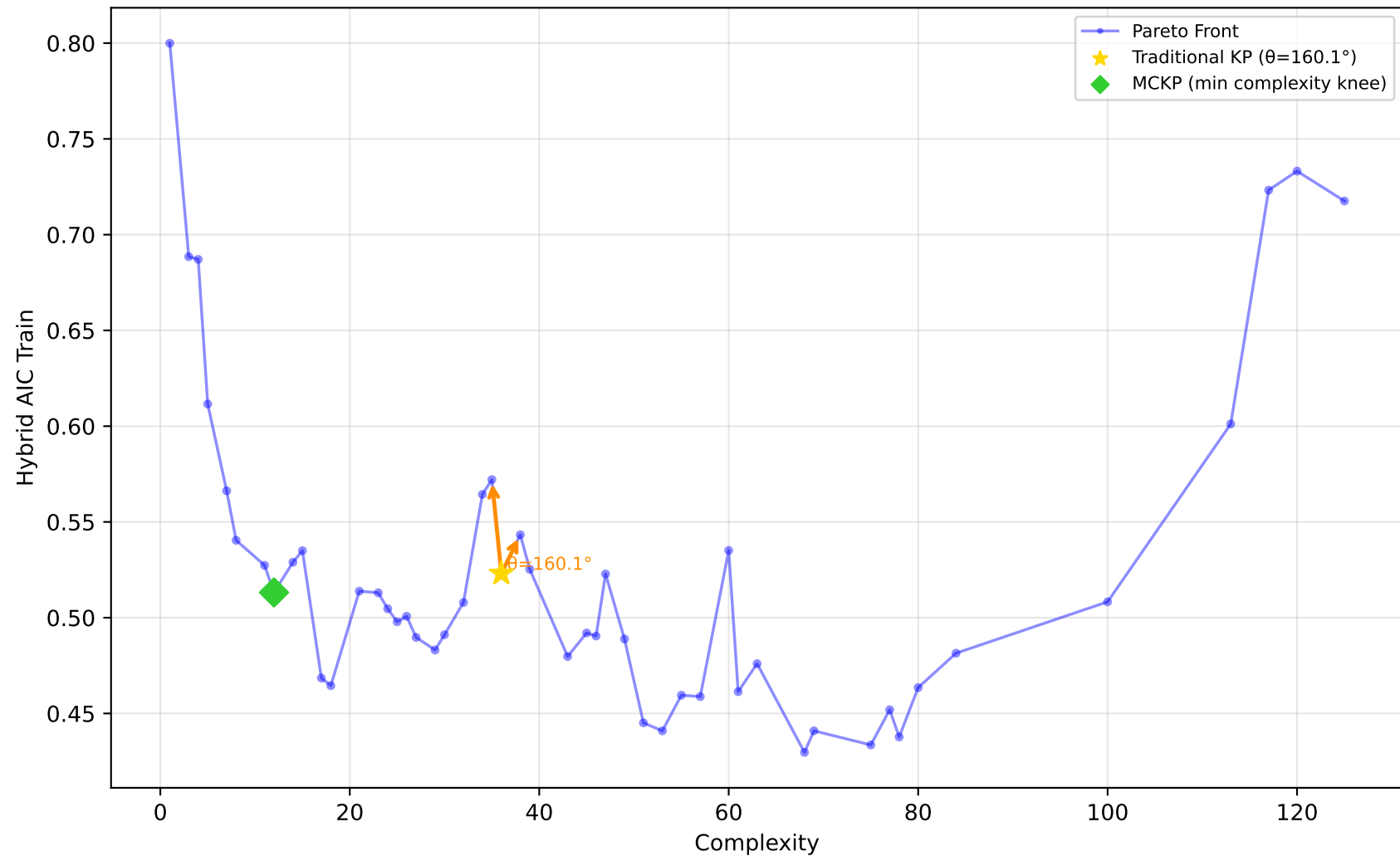
192_vineyard - Run 2 - SVP - Hybrid AIC Train \lambda_1=0.00, \lambda_2=1.00, \lambda_3=1.00 | Difficulty: 0.13 | Method: mckp
