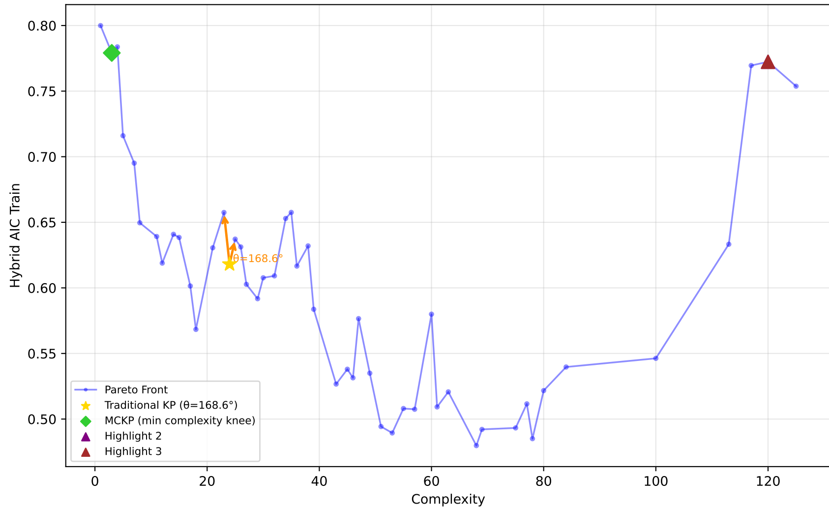
192_vineyard - Run 2 - SVP - Hybrid AIC Train \lambda_1=0.70, \lambda_2=0.70, \lambda_3=0.90 | Difficulty: 0.13 | Method: mckp
