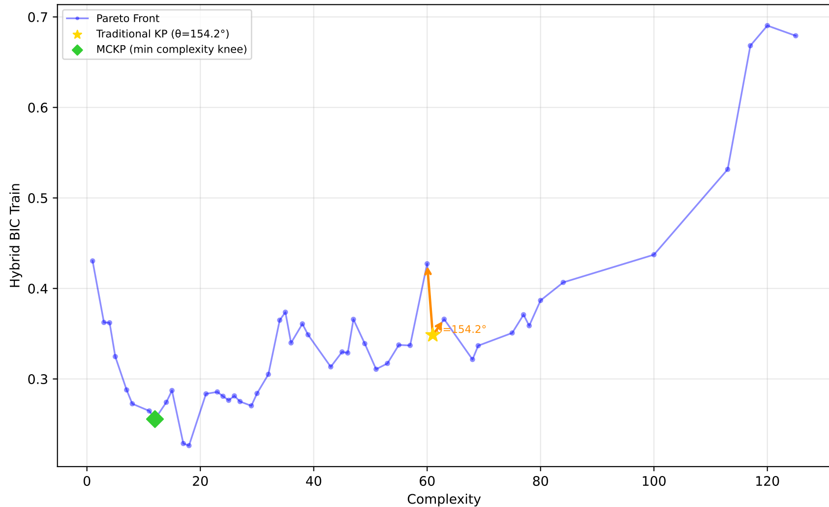
192_vineyard - Run 2 - SVP - Hybrid BIC Train \lambda_1=0.00, \lambda_2=1.00, \lambda_3=1.00 | Difficulty: 0.13 | Method: mckp
