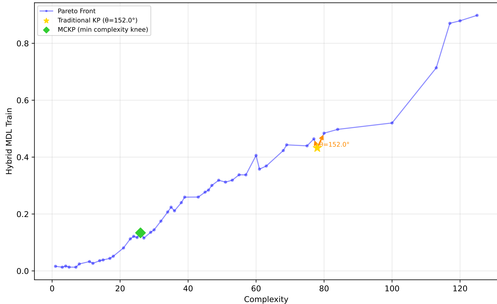
192_vineyard - Run 2 - SVP - Hybrid MDL Train \lambda_1=0.00, \lambda_2=1.00, \lambda_3=1.00 | Difficulty: 0.13 | Method: mckp
