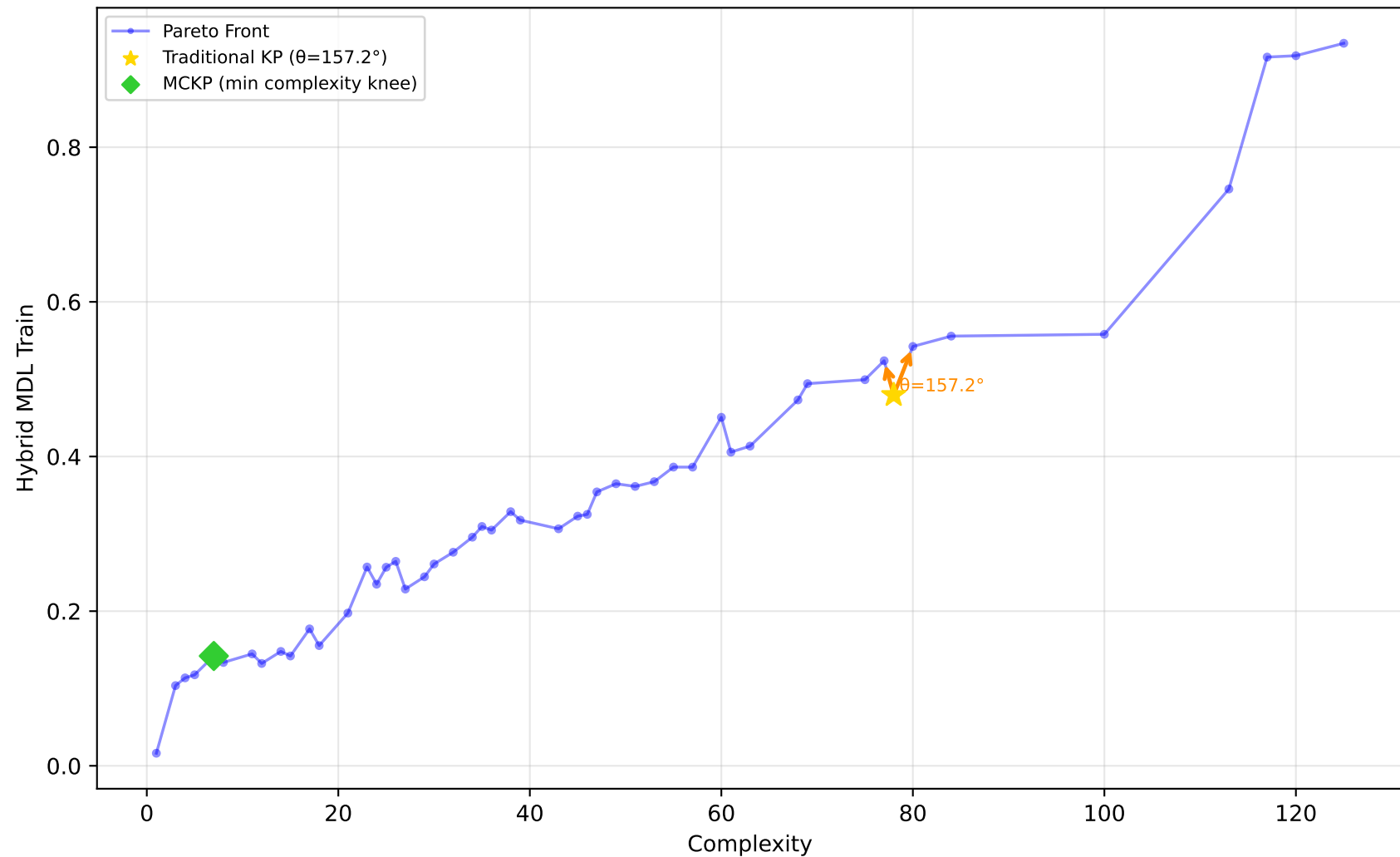
192_vineyard - Run 2 - SVP - Hybrid MDL Train \lambda_1=0.70, \lambda_2=0.70, \lambda_3=0.90 | Difficulty: 0.13 | Method: mckp
