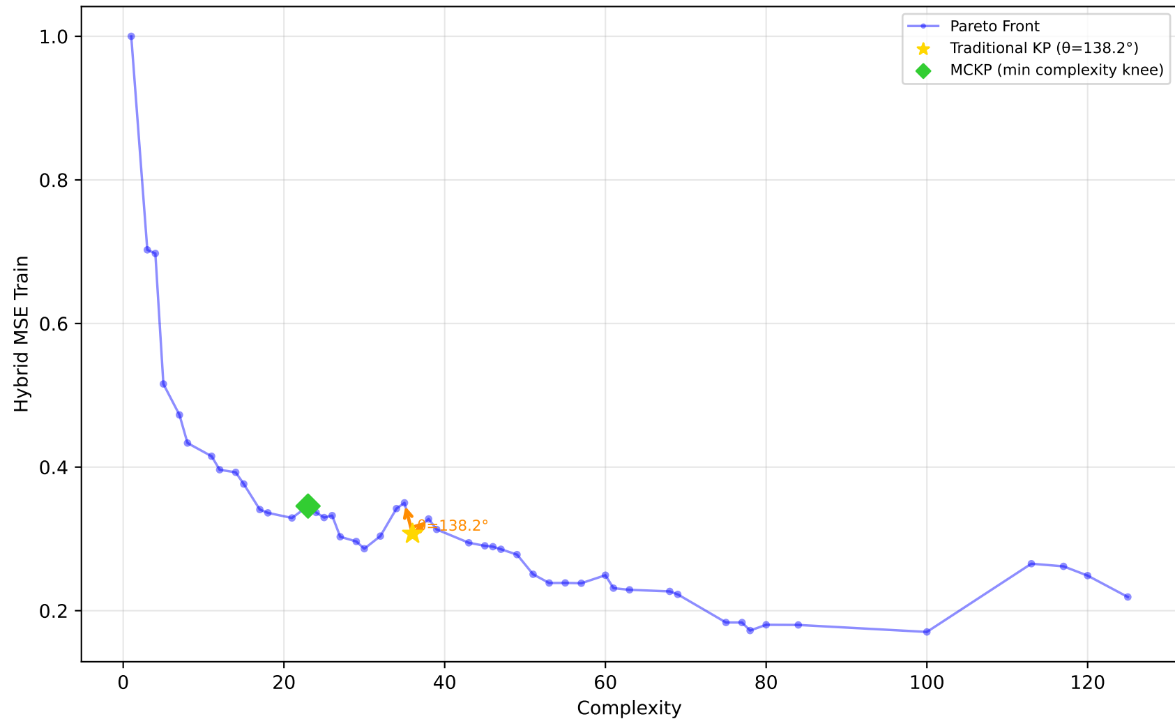
192_vineyard - Run 2 - SVP - Hybrid MSE Train \lambda_1=0.00, \lambda_2=1.00, \lambda_3=1.00 | Difficulty: 0.13 | Method: mckp
